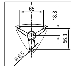
HD9008.31 Flange
