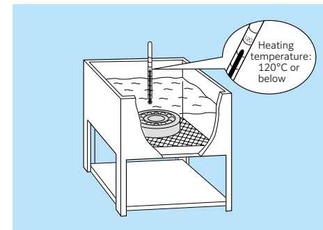
Fig. 15.16 Heating bearings in oil bath
