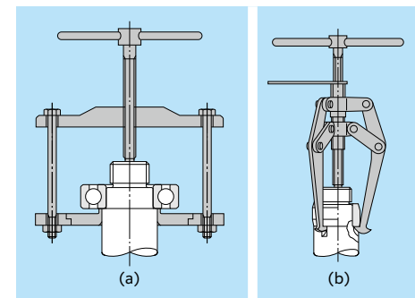
Fig. 15.28 Puller disassembly
