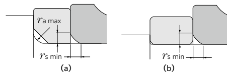
Fig. 14.1 Bearing mounting with spacer
