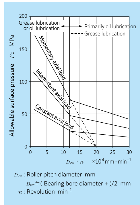
Fig. 3.16 Allowable surface pressure of rib
