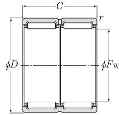
RNA69 type · R type ( \phi F_w \geq 40\text{mm} )
