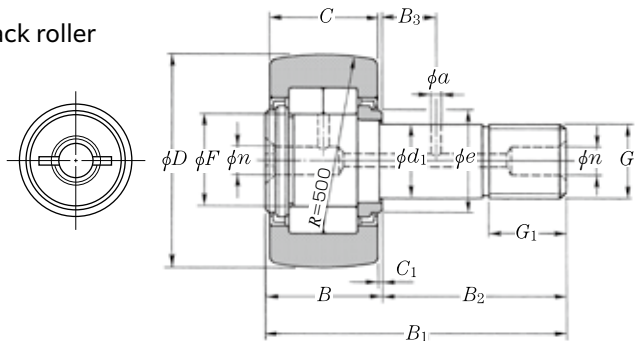
NUKR type ( D < 100 \text{ mm} ) (Full complement double-row cylindrical roller bearings with shield)
