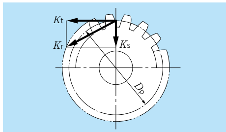
Fig. 4.3 Radial resultant forces
