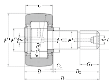
NUKR type ( D \geq 100 \text{ mm} )
