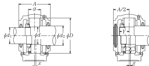
Shaft penetration type
