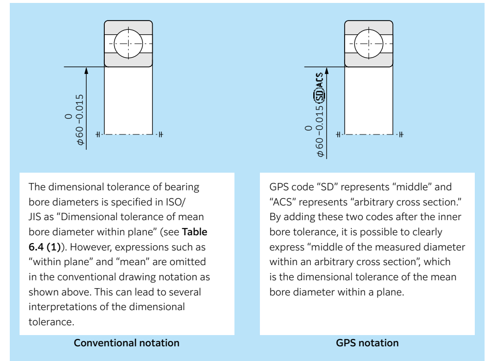
Fig. 6.2 Notation example of bearing bore diameter tolerance
