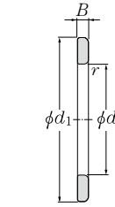
WS type raceway (Inner ring)
