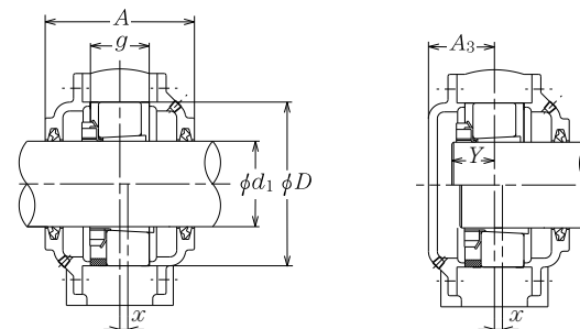
Shaft penetration type
