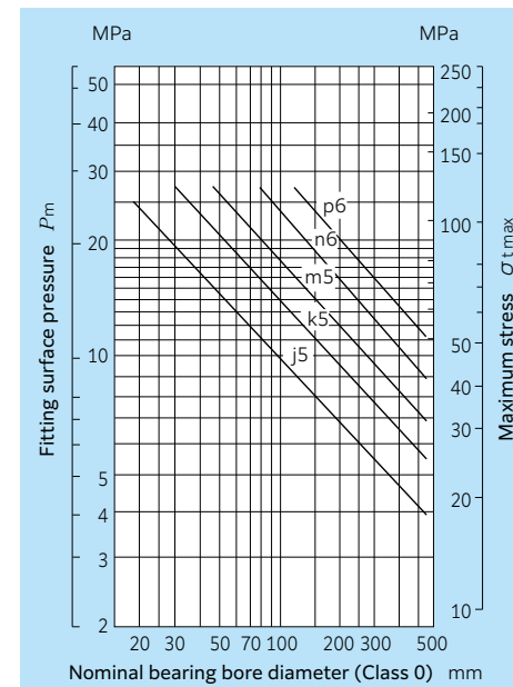
Fig. 17.4.2 Maximum fit interference as it relates to surface pressure P_m and maximum stress \sigma_{t \max}
