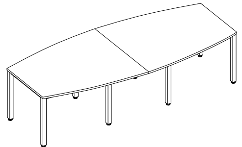
2400, 2800 × 1200/800 × 740 mm, 3200, 3600, 4000 × 1400/1000 × 740 mm
