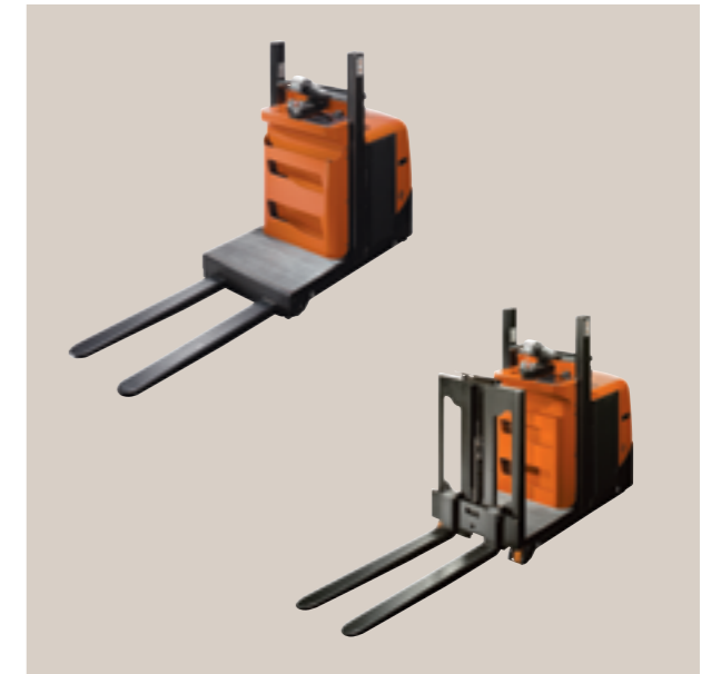
OSE100W / OSE100 • Max. capacity 1000 kg • Elevating platform up to 1.2 m for lower-intensity man-up picking • On OSE100, initial lift allows the load carrier to be elevated for comfortable operation
